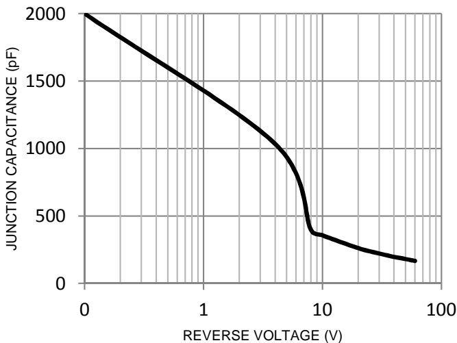
FIG. 5-Typical Junction Capacitance
