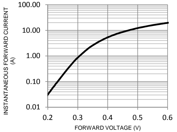
FIG. 2-Typical Forward Characteristics
